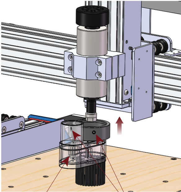
Dust Shoe M6x6 Screws
